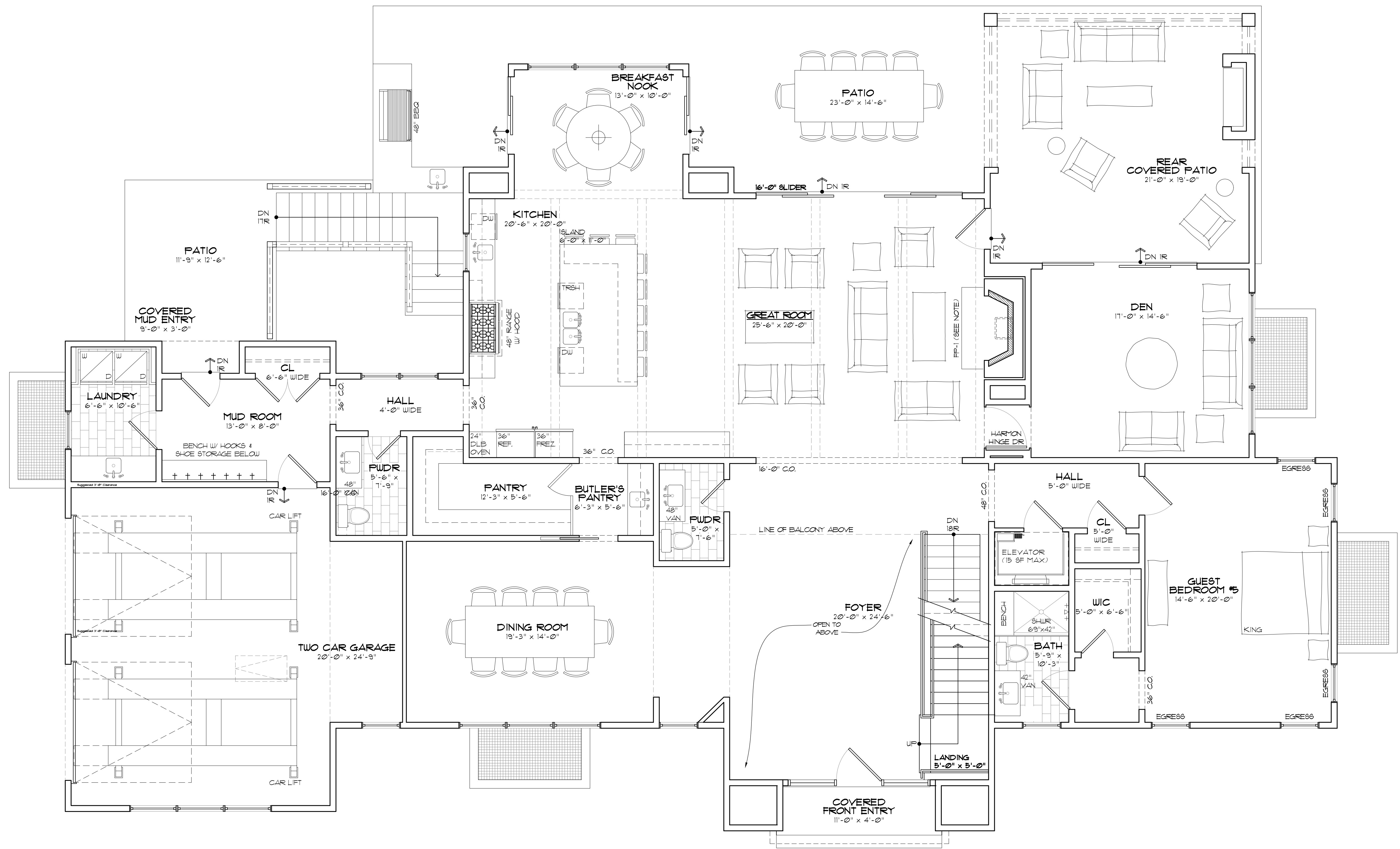
1 A-101 PROPOSED FIRST FLOOR PLAN
