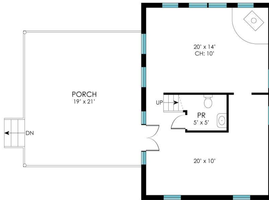
1ST FLOOR
