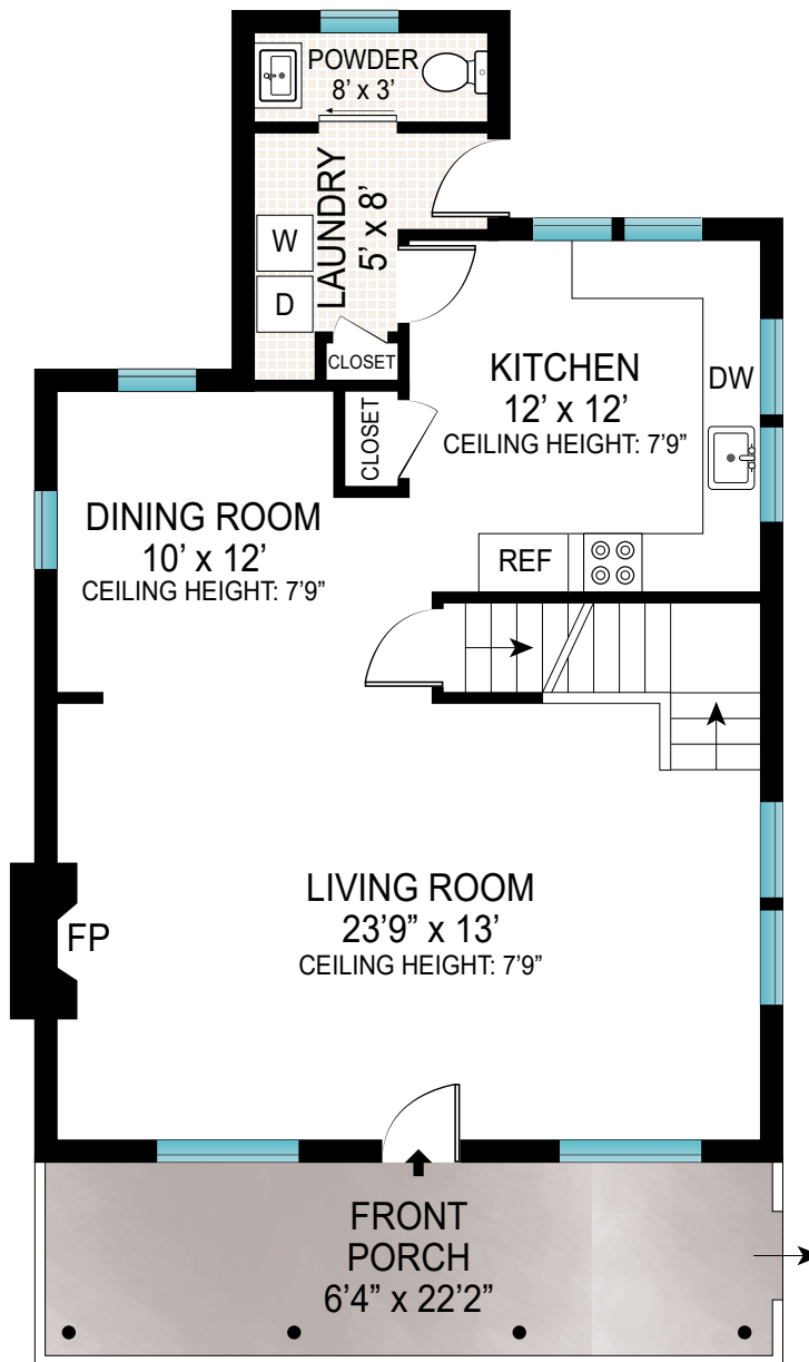
FIRST FLOOR CEILING HEIGHT: 7'9"
