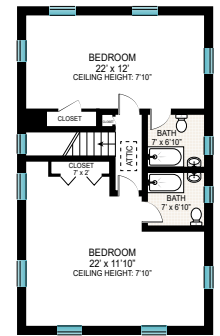
SECOND FLOOR (GUEST HOUSE)
