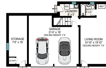
FIRST FLOOR (COTTAGE)
