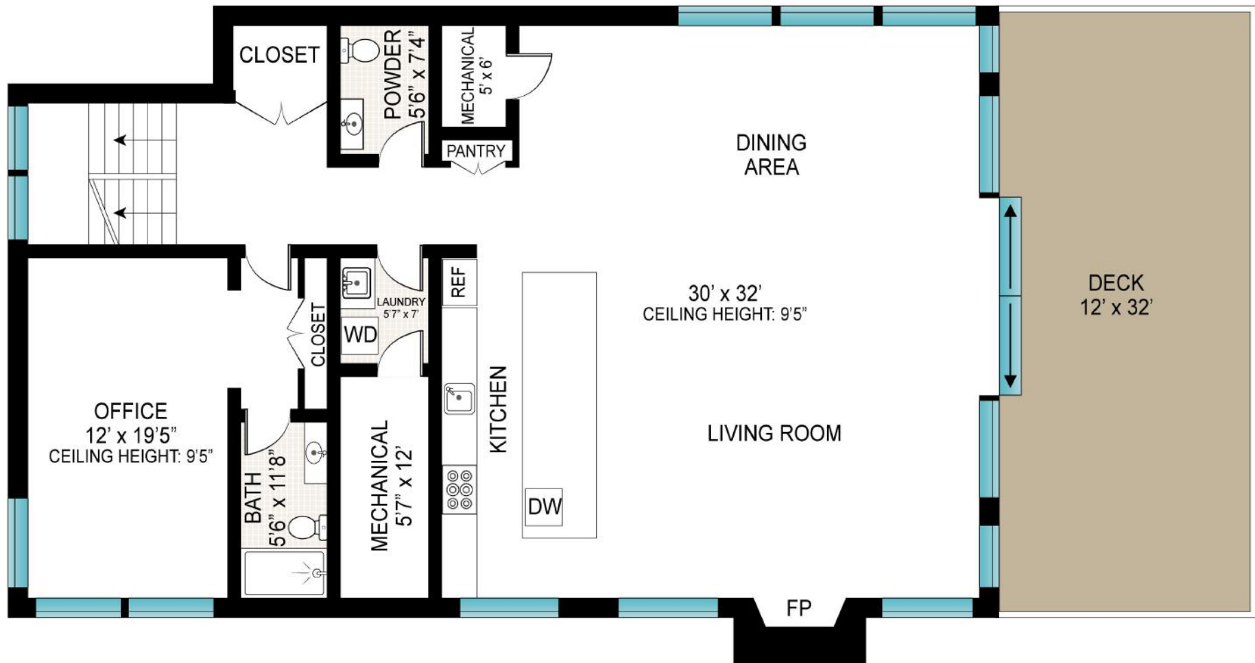
SECOND FLOOR CEILING HEIGHT: 9'5"
