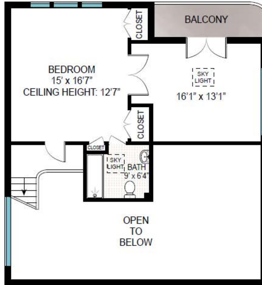
SECOND FLOOR CEILING HEIGHT: 12'7"
