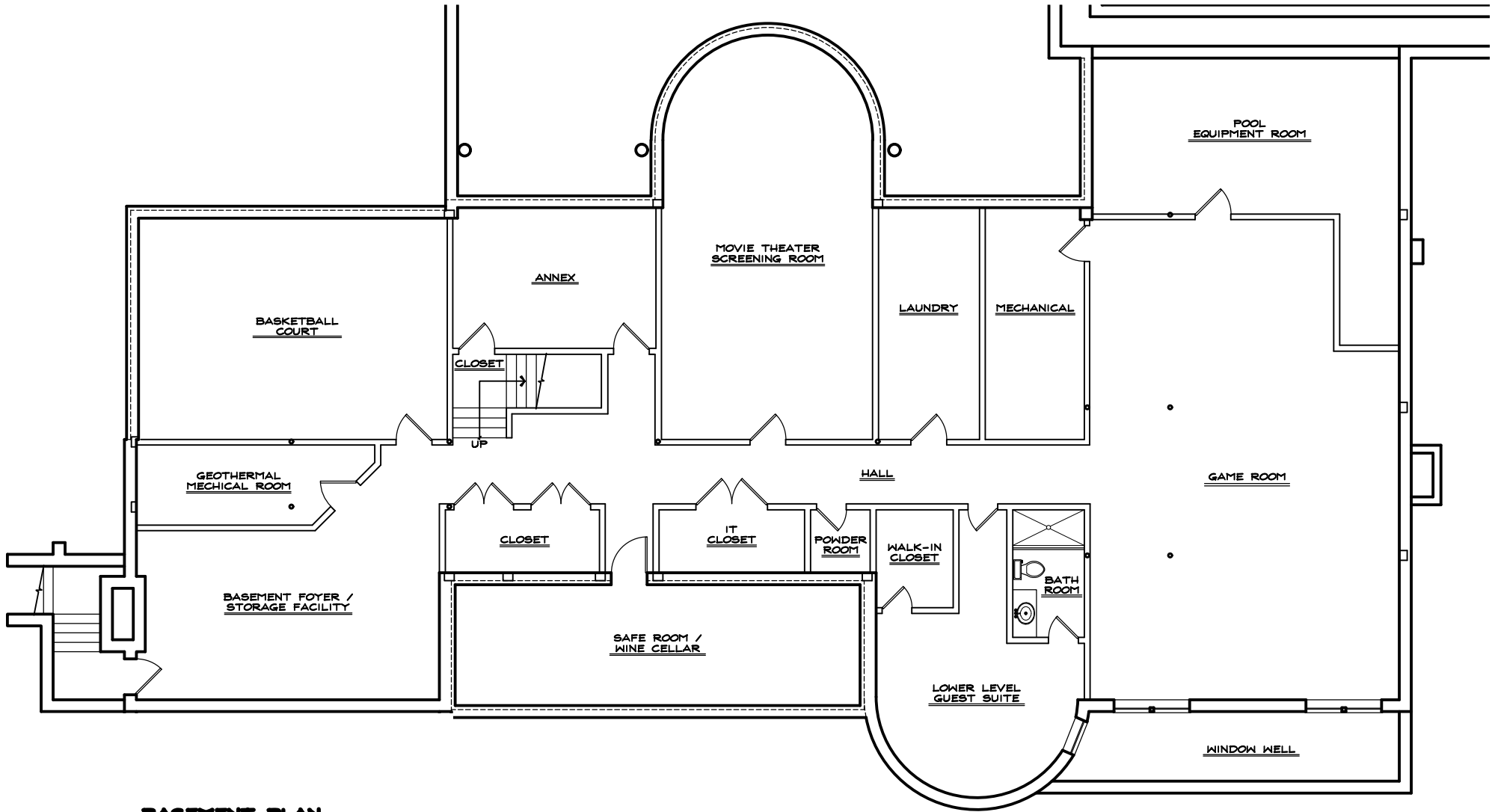
BASEMENT PLAN SCALE: 1/4"=1'-0"
